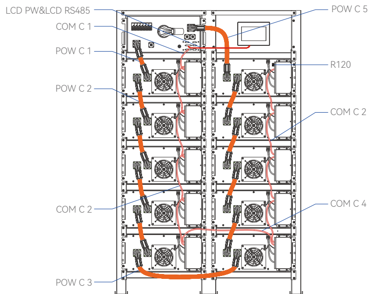
Wiring diagram
